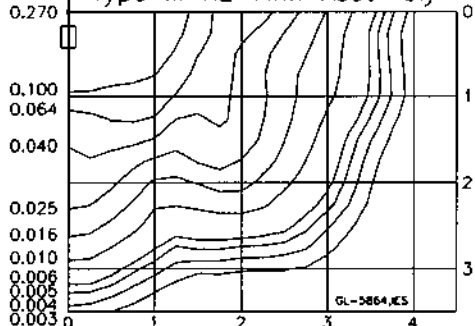
METAL HALIDE Type III XL Twin Assembly
