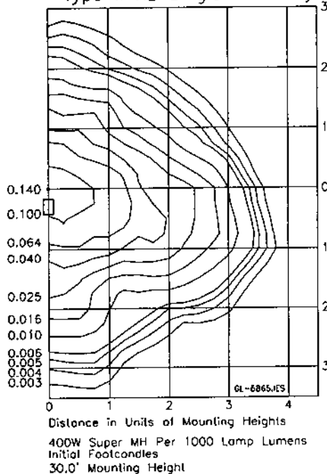
METAL HALIDE Type II XL Single Assembly
