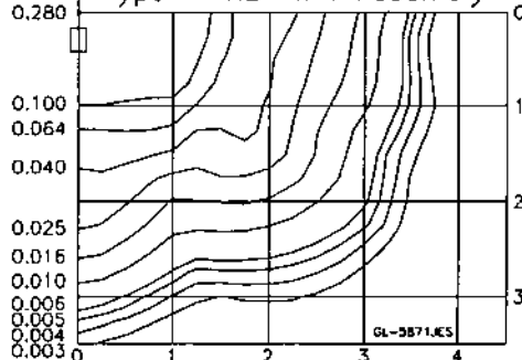
HIGH PRESSURE SODIUM Type III XL Twin Assembly
