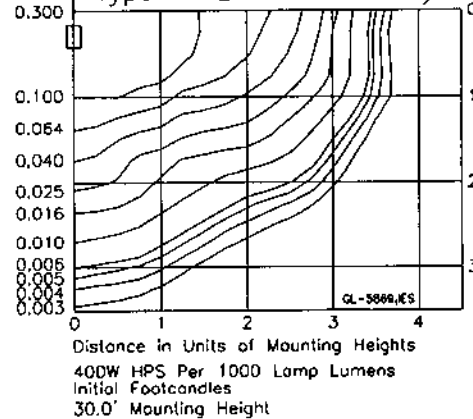
HIGH PRESSURE SODIUM Type II XL Twin Assembly
