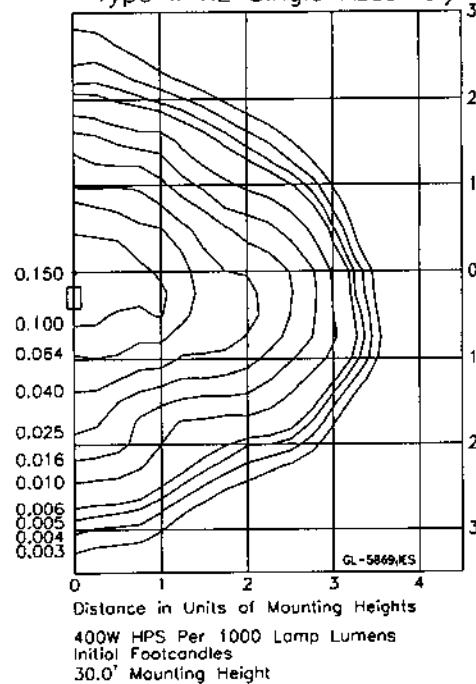
HIGH PRESSURE SODIUM Type II XL Single Assembly
