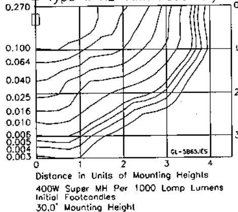
METAL HALIDE Type II XL Twin Assembly
