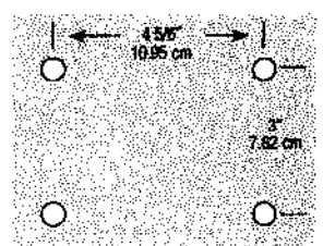
Mounting Bracket Pattern
