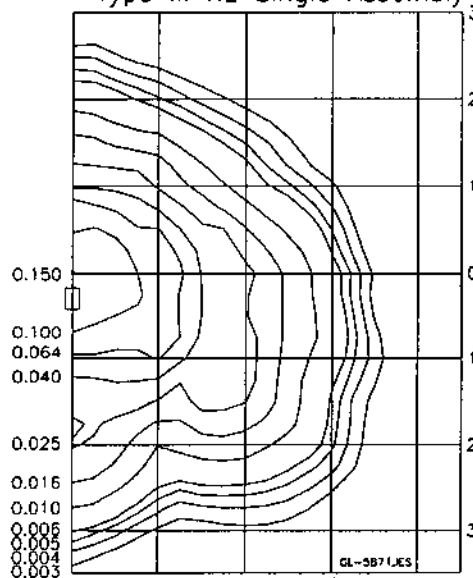
HIGH PRESSURE SODIUM Type III XL Single Assembly
