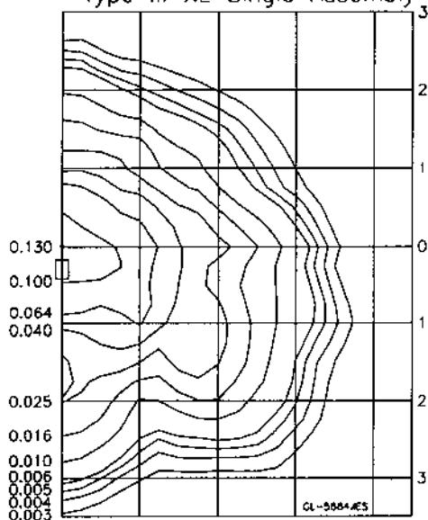
METAL HALIDE Type III XL Single Assembly
